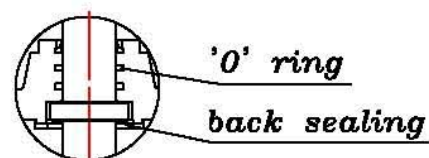
Packing detail
